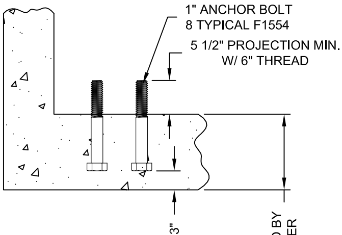
TYPICAL ANCHOR BOLT
