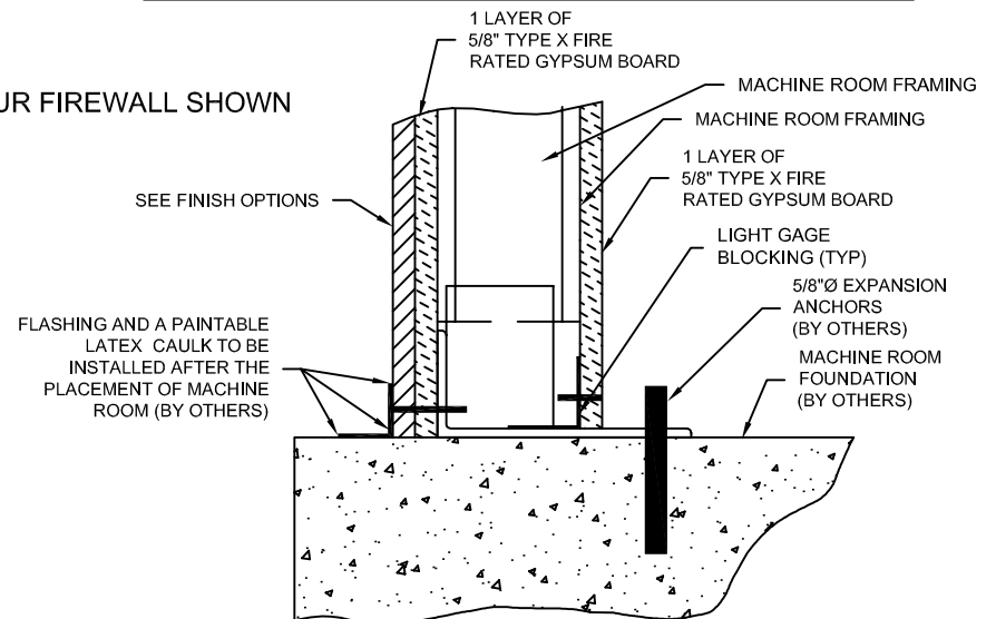
H - MACHINE ROOM FLASHING DETAIL
