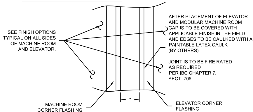
G - MACHINE ROOM & ELEVATOR DETAIL
