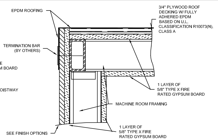
F - MACHINE ROOM ROOF DETAIL
