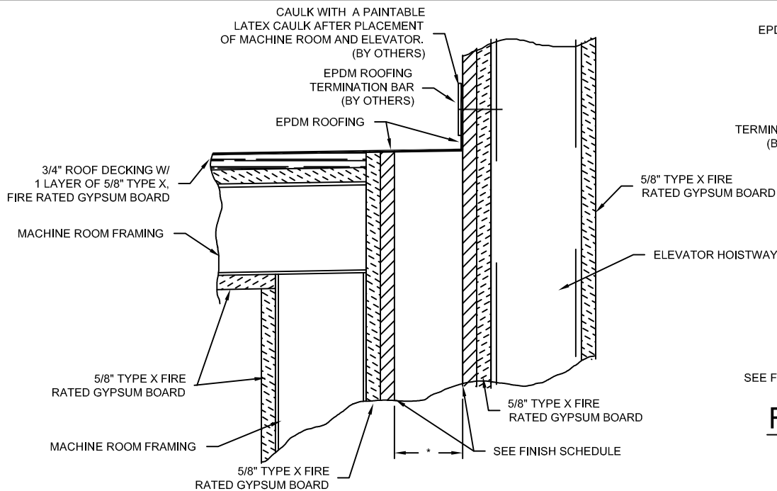
E - MACHINE ROOM ROOF DETAIL WITH ELEVATOR
