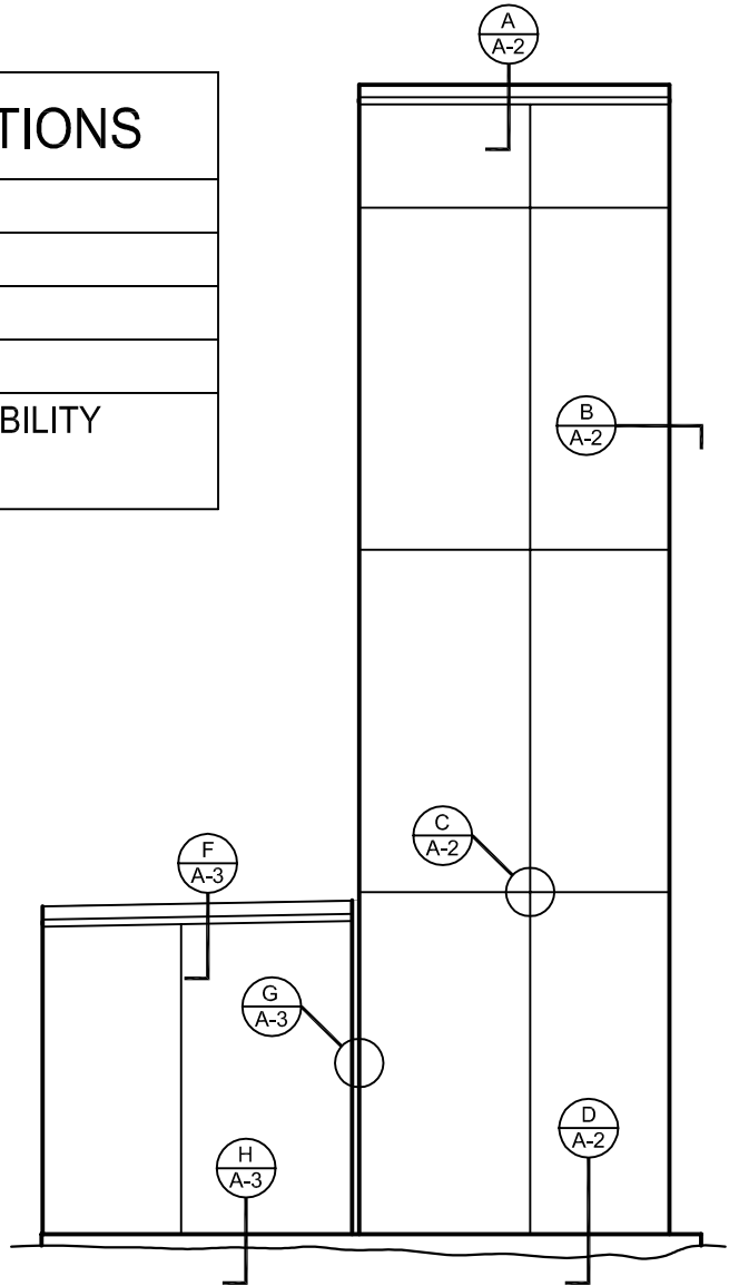
SIDE ELEVATION MODULAR ELEVATOR AND (OPTIONAL) MODULAR MACHINE ROOM FIREWALL SYSTEM
