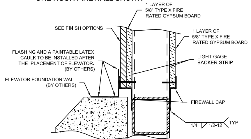
D - ELEVATOR HOISTWAY FLASHING DETAIL ONE HOUR FIREWALL SHOWN
