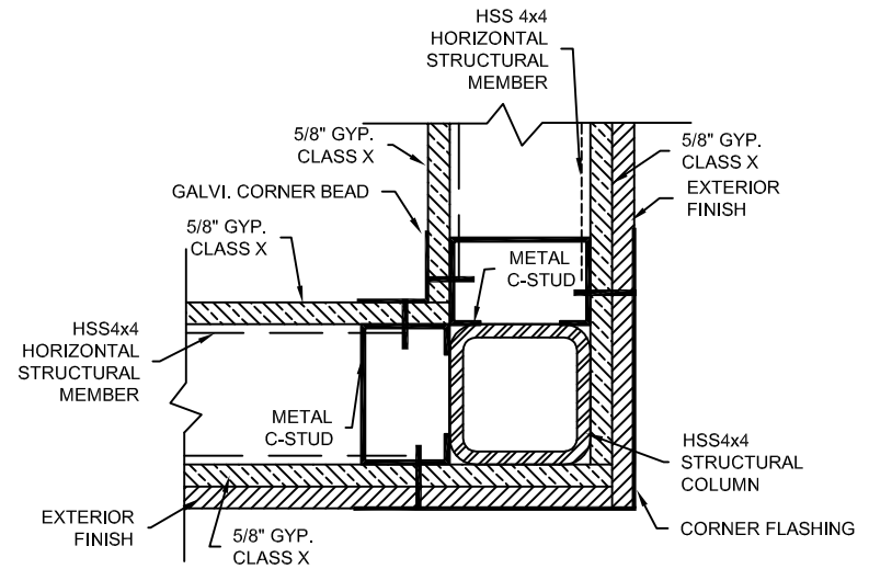
B - ELEVATOR HOISTWAY CORNER DETAIL ONE HOUR FIREWALL SHOWN
