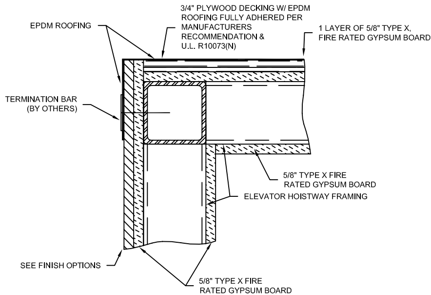
A - ELEVATOR HOISTWAY ROOF DETAIL ONE HOUR FIREWALL SHOWN
