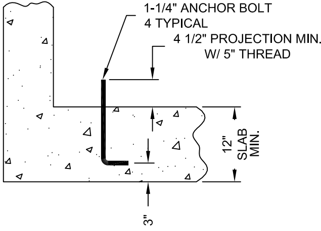
TYPICAL ANCHOR BOLT
